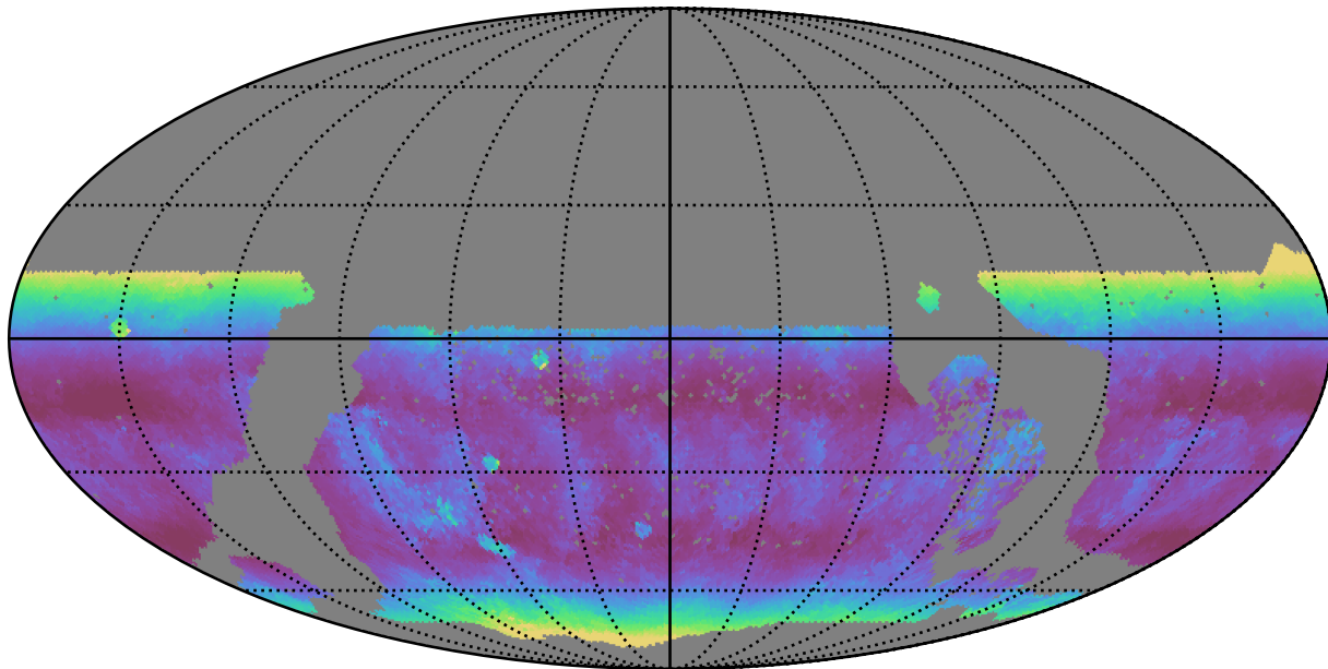
ddf_loaded_fl15_v3.4_10yrs WFD u band: Median airmass
