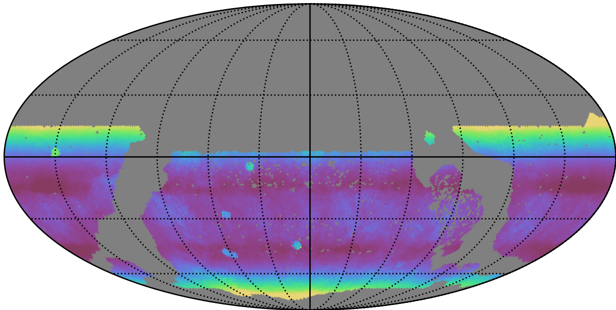
ddf_loaded_fl15_v3.4_10yrs WFD r band: Median airmass
