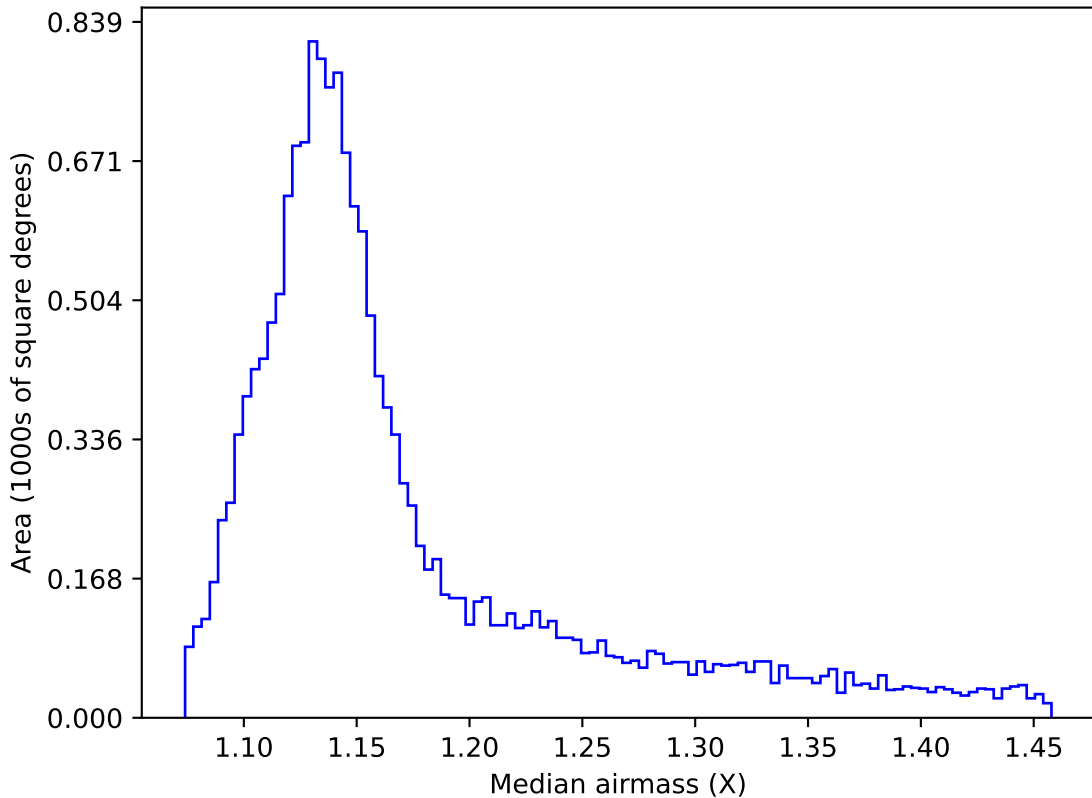
ddf_loaded_fl15_v3.4_10yrs WFD r band: Median airmass
