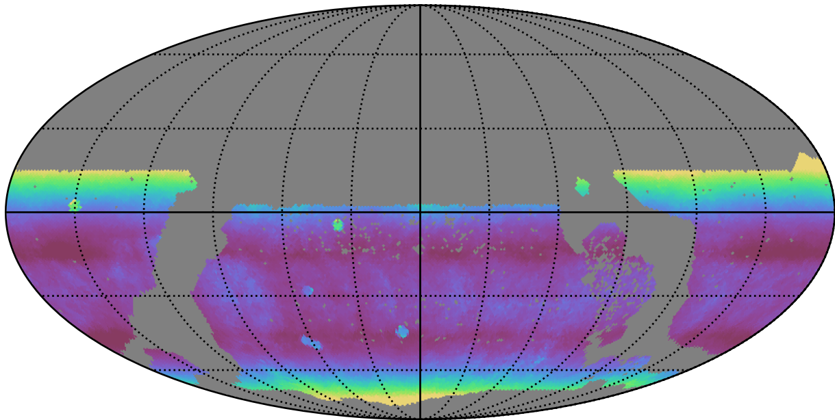
ddf_loaded_fl15_v3.4_10yrs WFD i band: Median airmass
