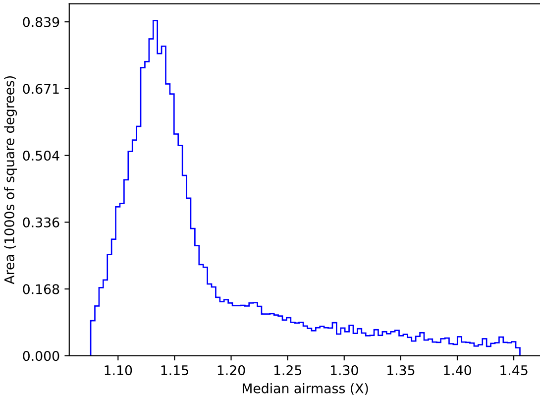
ddf_loaded_fl15_v3.4_10yrs WFD i band: Median airmass
