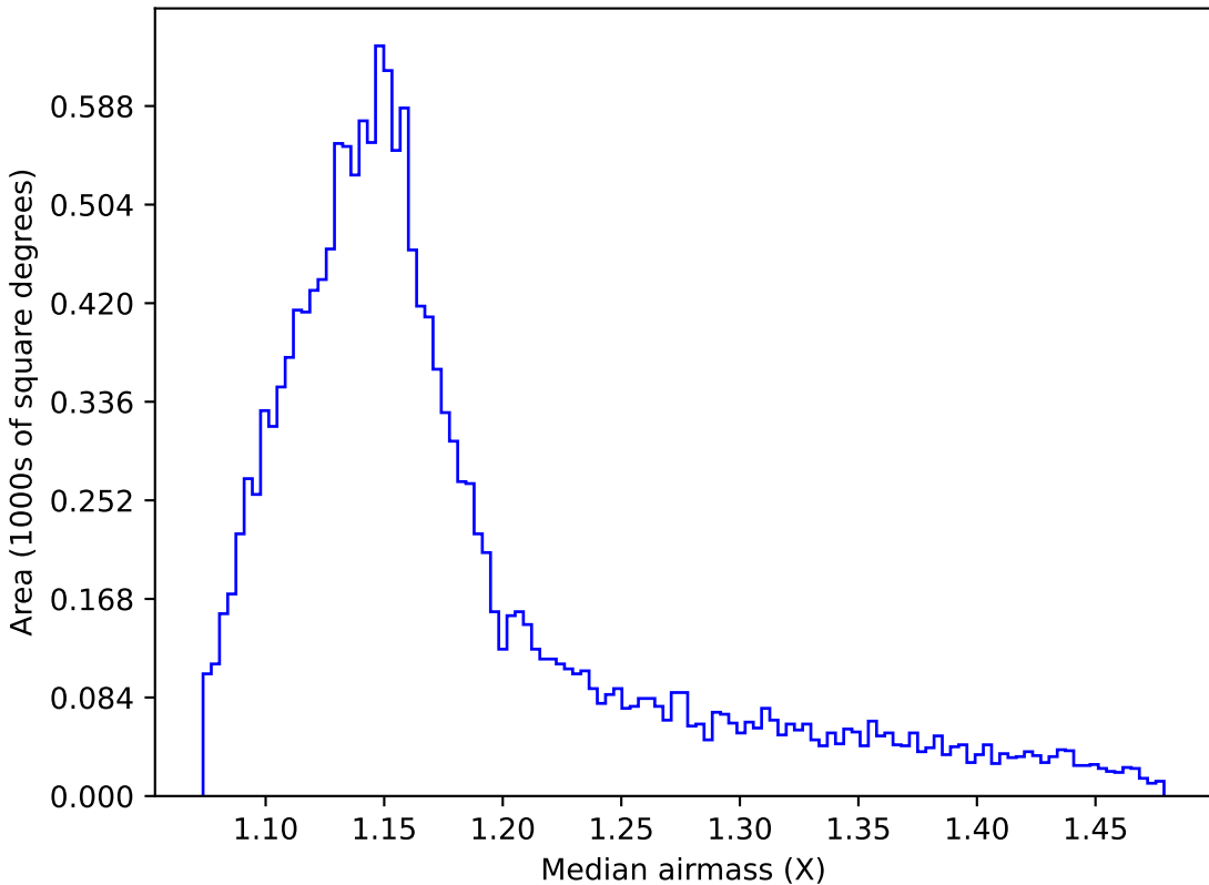
ddf_loaded_fl15_v3.4_10yrs WFD g band: Median airmass
