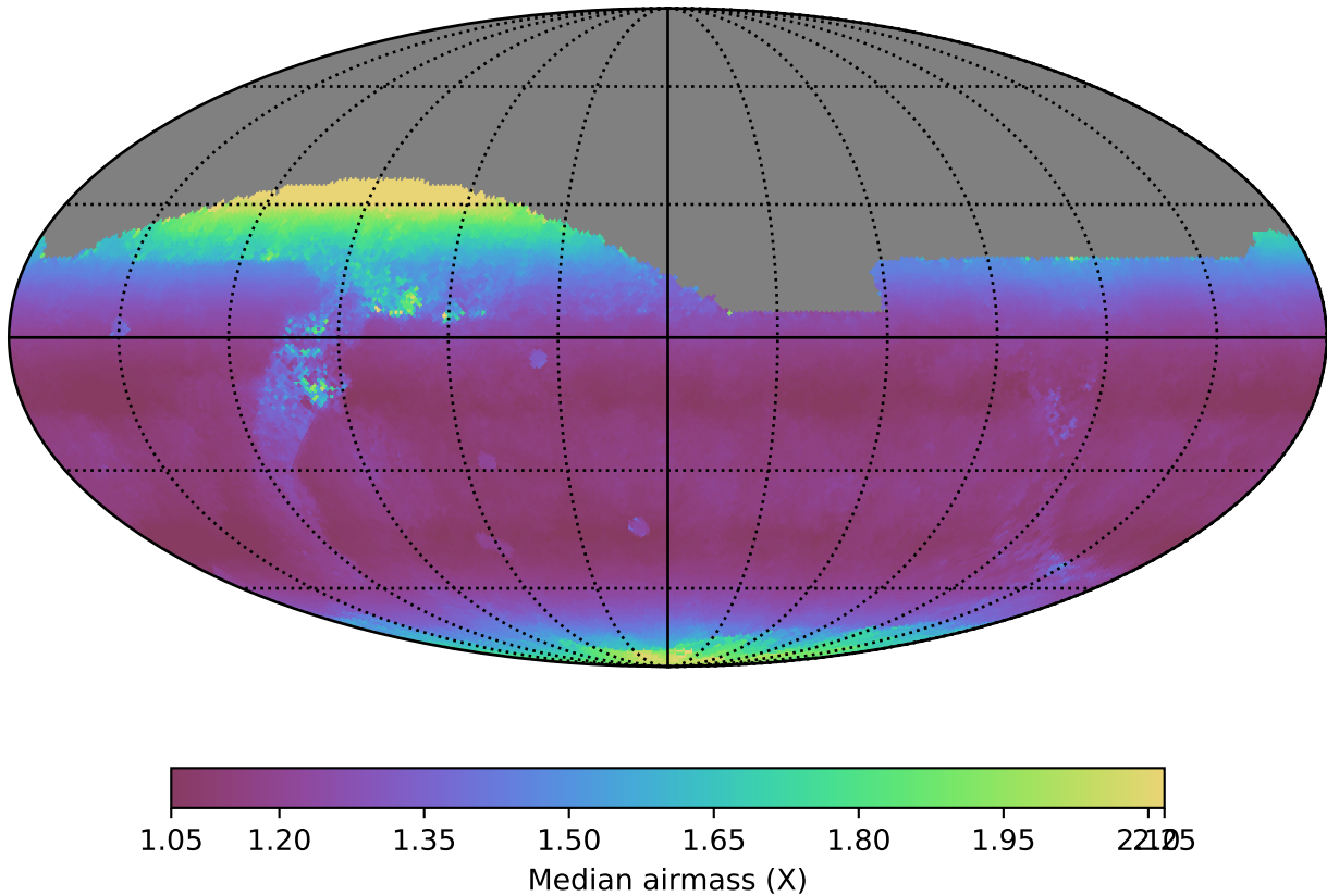
ddf_loaded_fl15_v3.4_10yrs All sky z band: Median airmass
