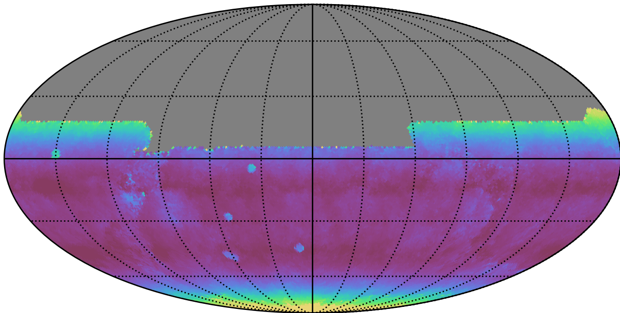
ddf_loaded_fl15_v3.4_10yrs All sky y band: Median airmass
