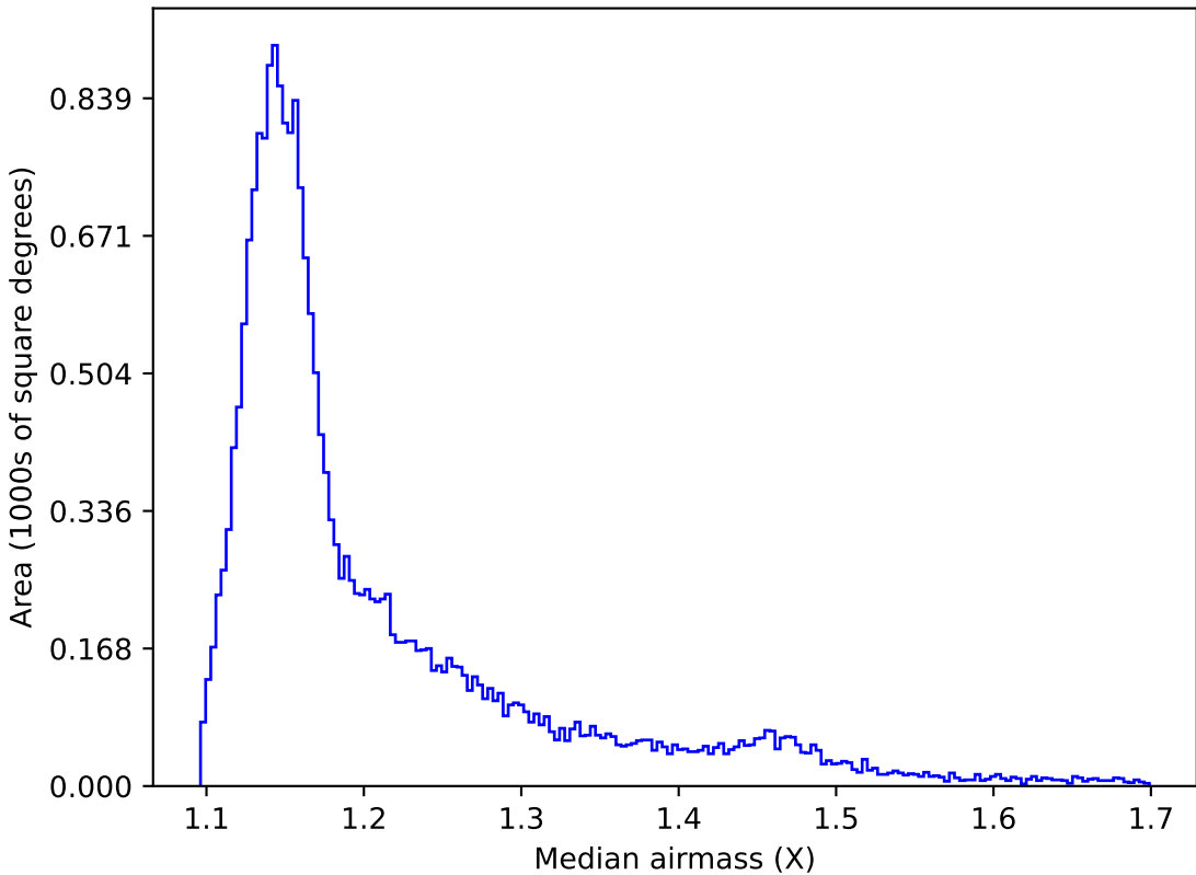
ddf_loaded_fl15_v3.4_10yrs All sky y band: Median airmass
