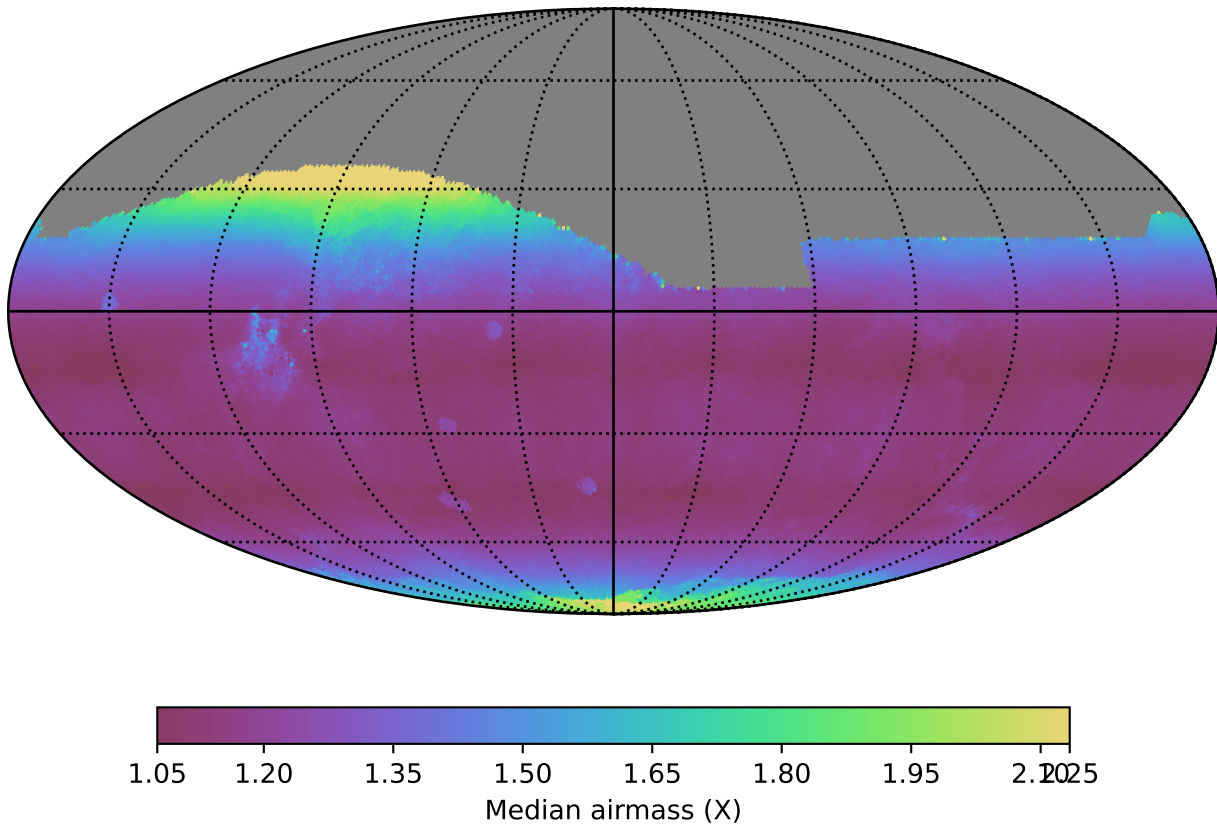
ddf_loaded_fl15_v3.4_10yrs All sky r band: Median airmass
