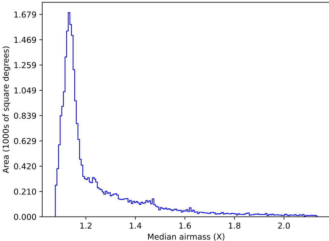
ddf_loaded_fl15_v3.4_10yrs All sky r band: Median airmass
