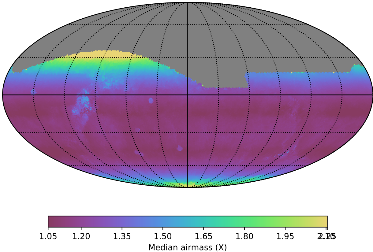
ddf_loaded_fl15_v3.4_10yrs All sky i band: Median airmass
