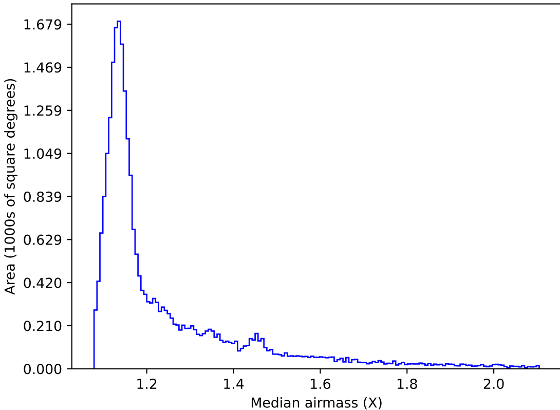
ddf_loaded_fl15_v3.4_10yrs All sky i band: Median airmass
