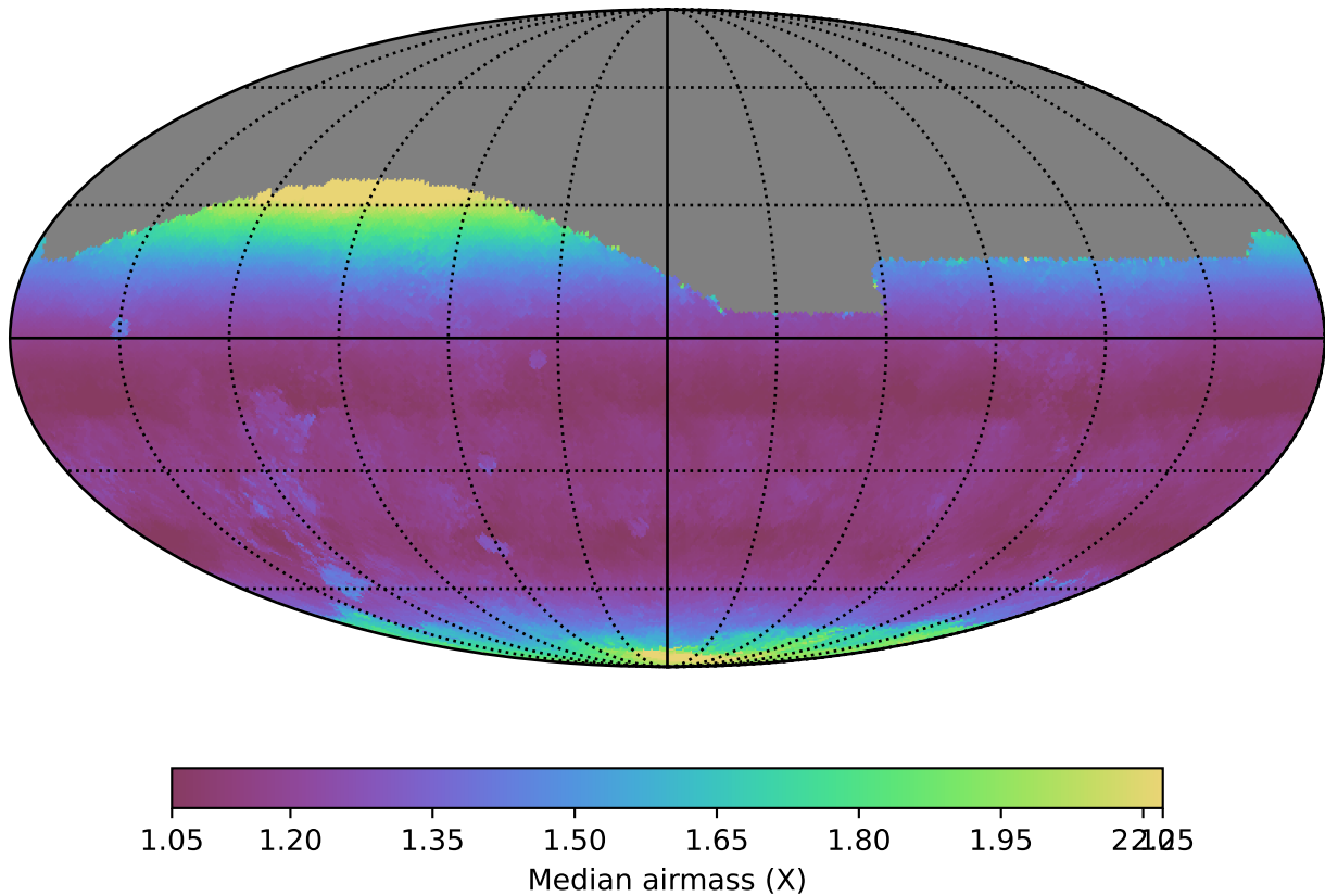
ddf_loaded_fl15_v3.4_10yrs All sky g band: Median airmass
