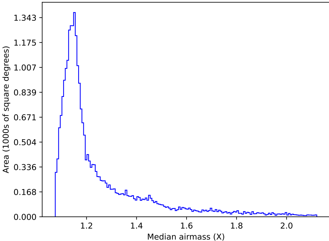
ddf_loaded_fl15_v3.4_10yrs All sky g band: Median airmass
