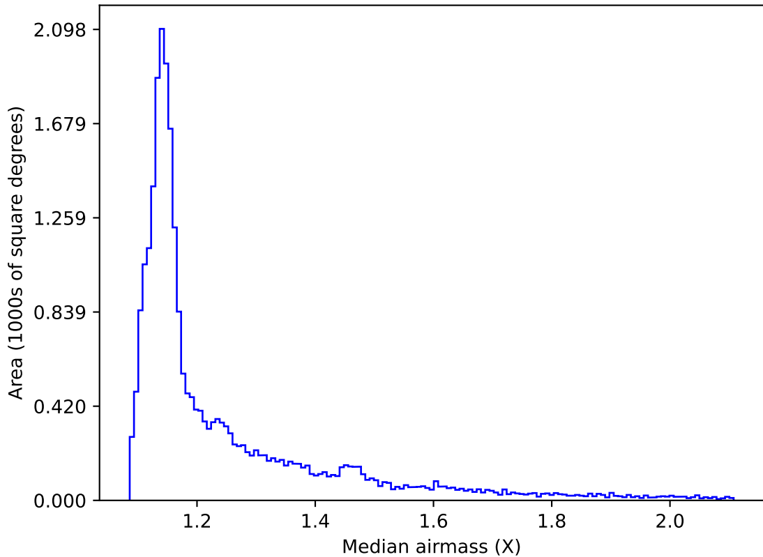
ddf_loaded_fl15_v3.4_10yrs All sky all bands: Median airmass
