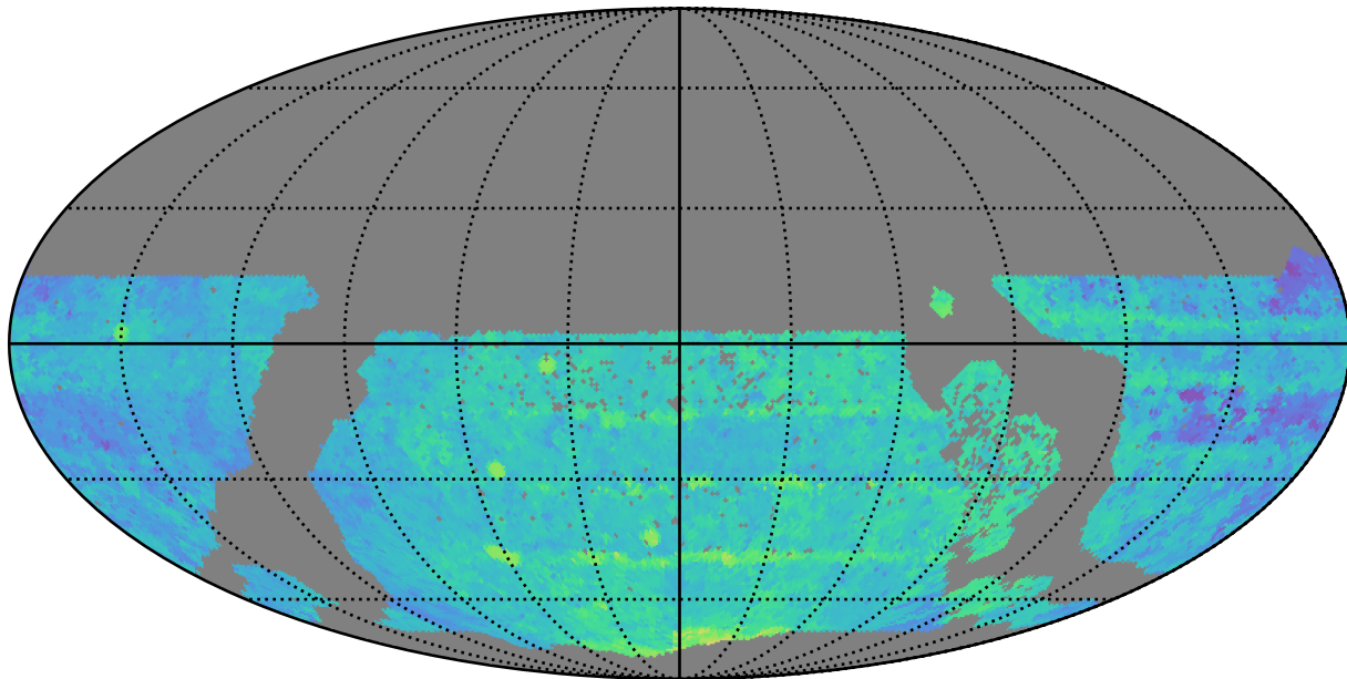
ddf_loaded_fl15_v3.4_10yrs WFD z band: Median Season Length
