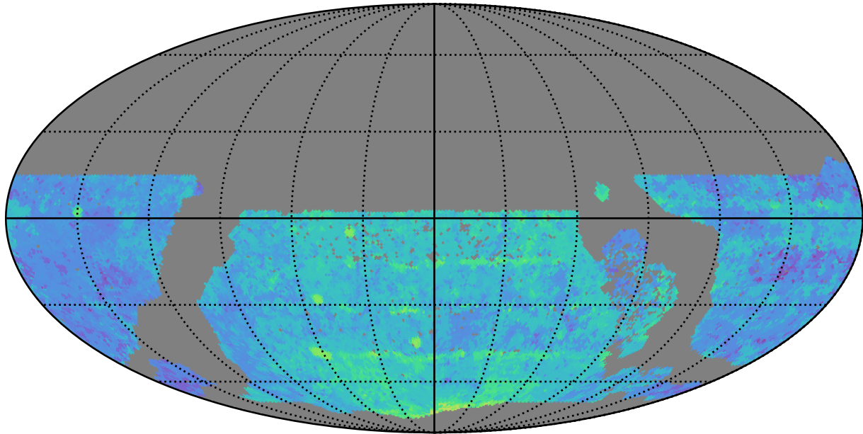
ddf_loaded_fl15_v3.4_10yrs WFD y band: Median Season Length
