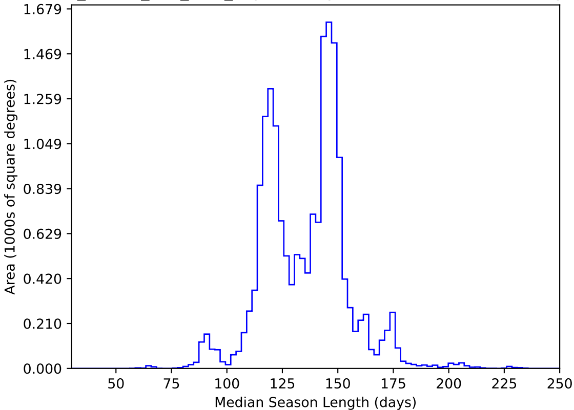
ddf_loaded_fl15_v3.4_10yrs WFD y band: Median Season Length
