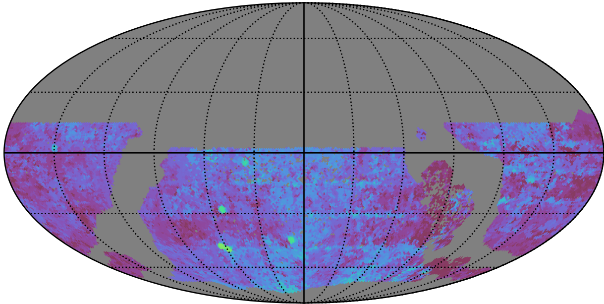
ddf_loaded_fl15_v3.4_10yrs WFD u band: Median Season Length
