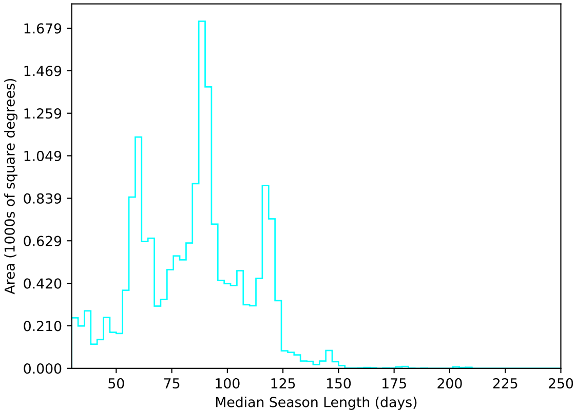
ddf_loaded_fl15_v3.4_10yrs WFD u band: Median Season Length
