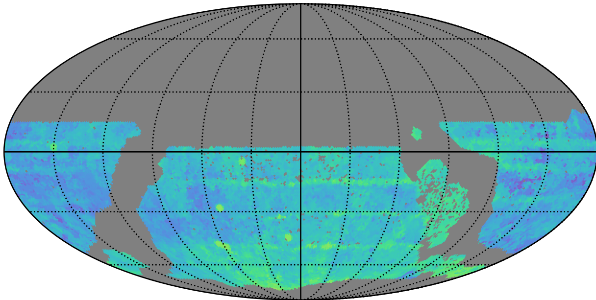
ddf_loaded_fl15_v3.4_10yrs WFD r band: Median Season Length
