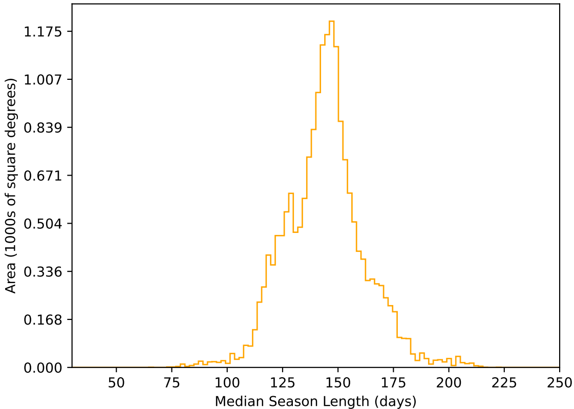
ddf_loaded_fl15_v3.4_10yrs WFD r band: Median Season Length
