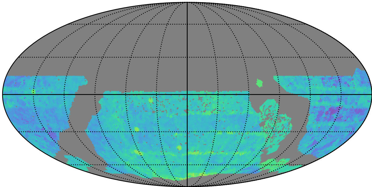
ddf_loaded_fl15_v3.4_10yrs WFD i band: Median Season Length
