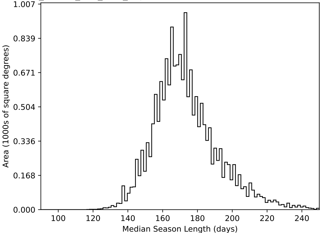
ddf_loaded_fl15_v3.4_10yrs WFD all bands: Median Season Length
