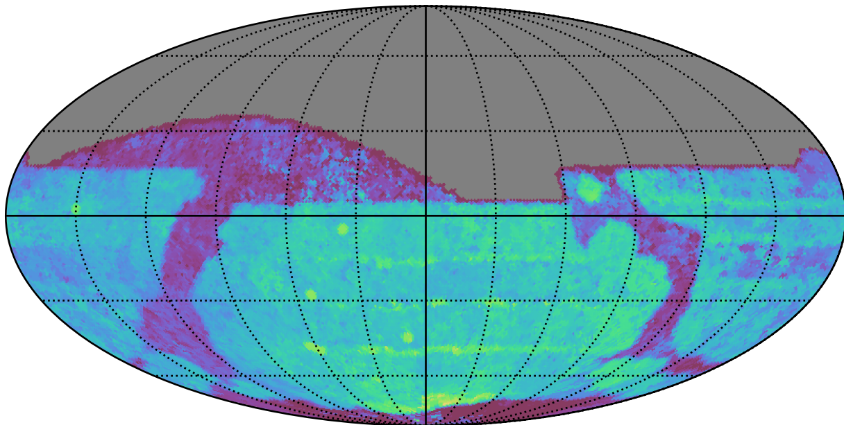
ddf_loaded_fl15_v3.4_10yrs All sky z band: Median Season Length
