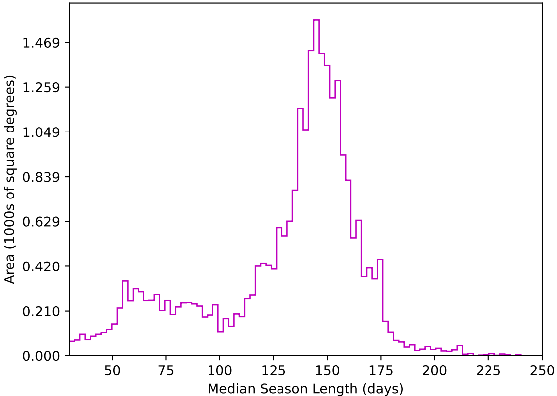
ddf_loaded_fl15_v3.4_10yrs All sky z band: Median Season Length
