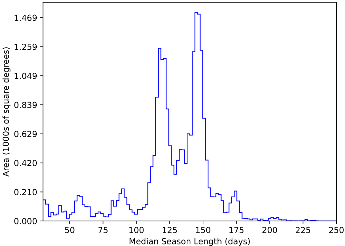
ddf_loaded_fl15_v3.4_10yrs All sky y band: Median Season Length
