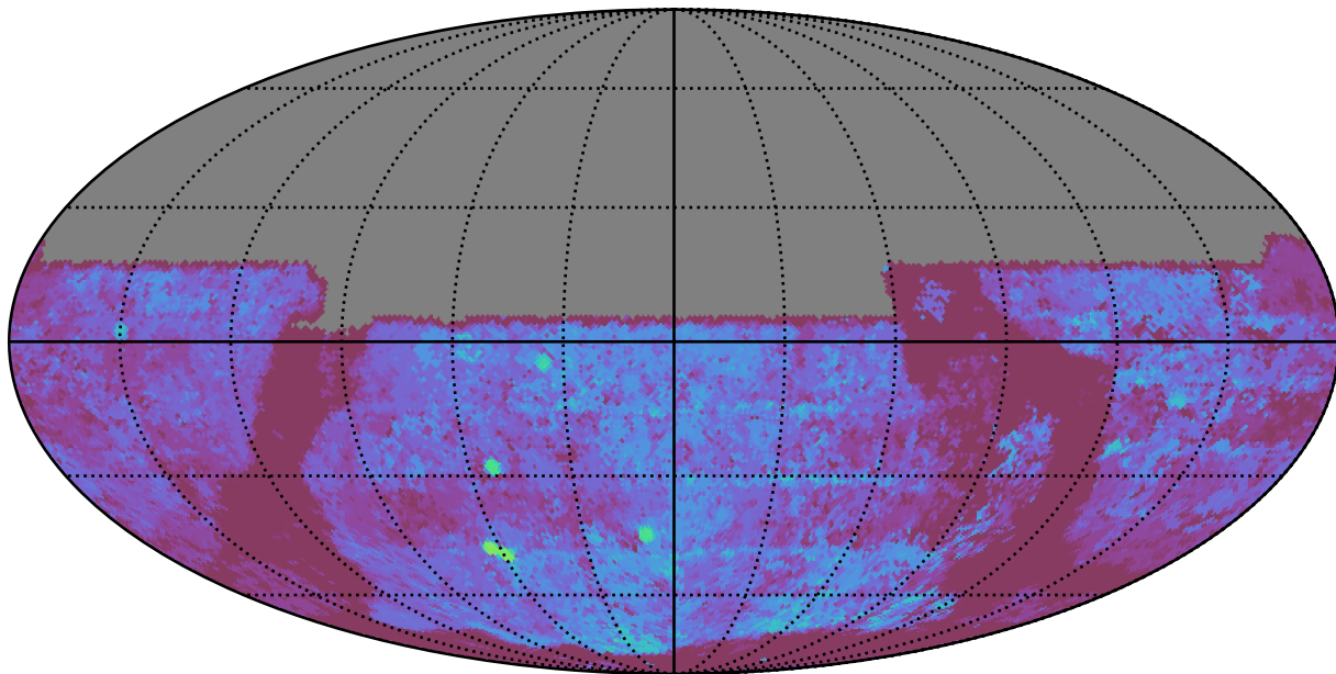
ddf_loaded_fl15_v3.4_10yrs All sky u band: Median Season Length
