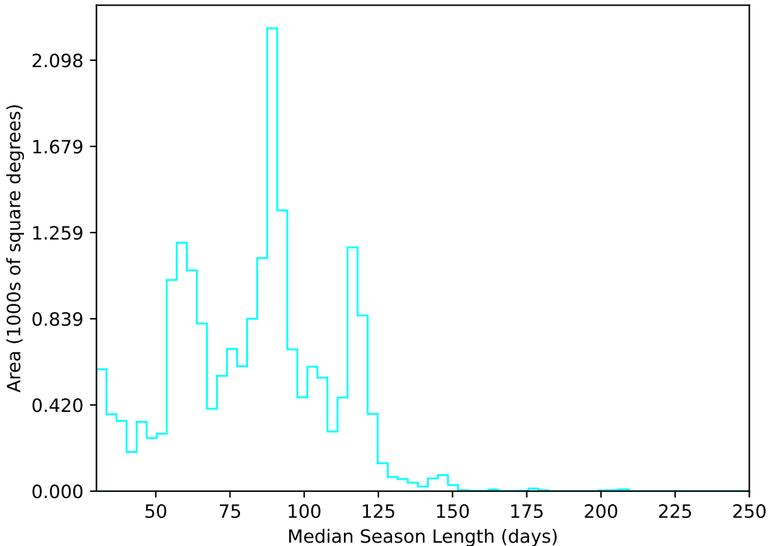
ddf_loaded_fl15_v3.4_10yrs All sky u band: Median Season Length
