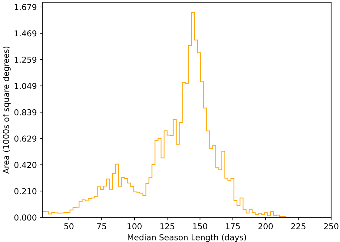
ddf_loaded_fl15_v3.4_10yrs All sky r band: Median Season Length
