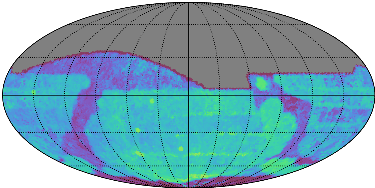
ddf_loaded_fl15_v3.4_10yrs All sky i band: Median Season Length
