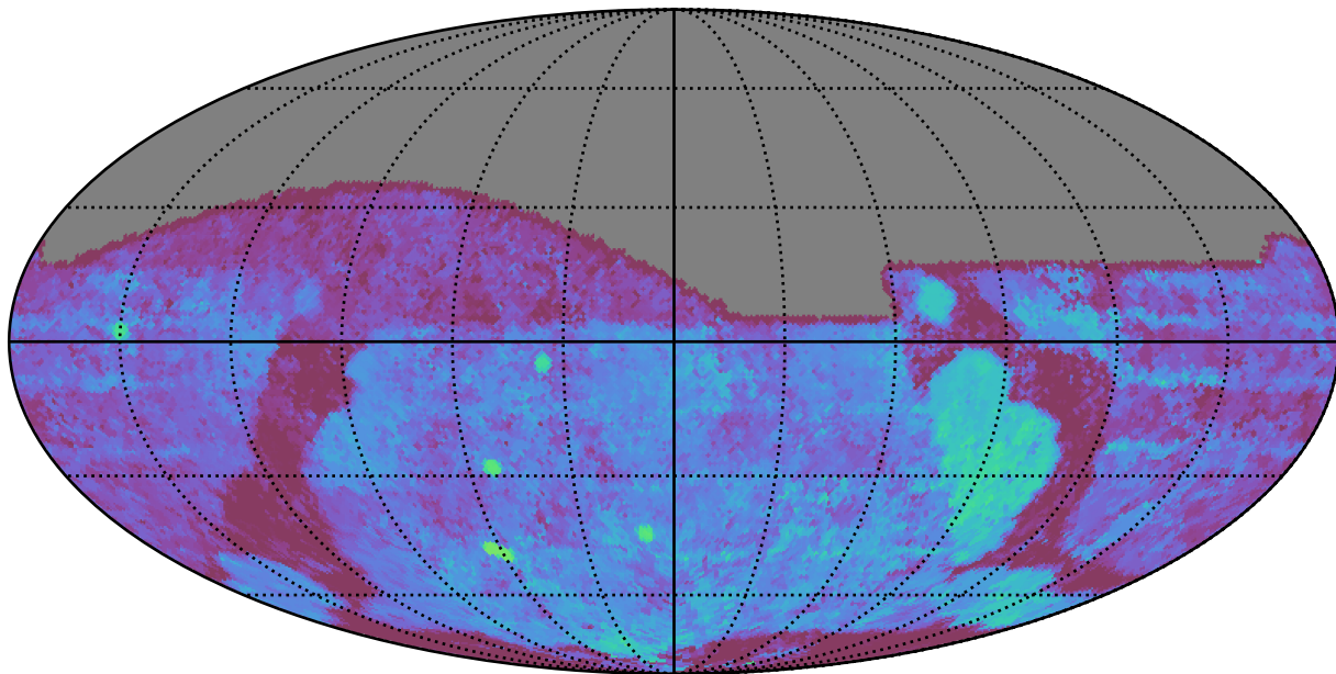
ddf_loaded_fl15_v3.4_10yrs All sky g band: Median Season Length
