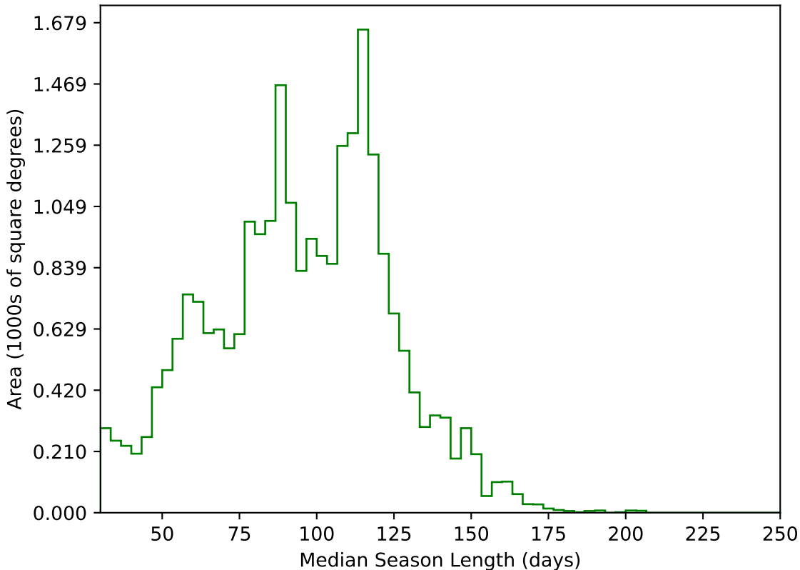
ddf_loaded_fl15_v3.4_10yrs All sky g band: Median Season Length
