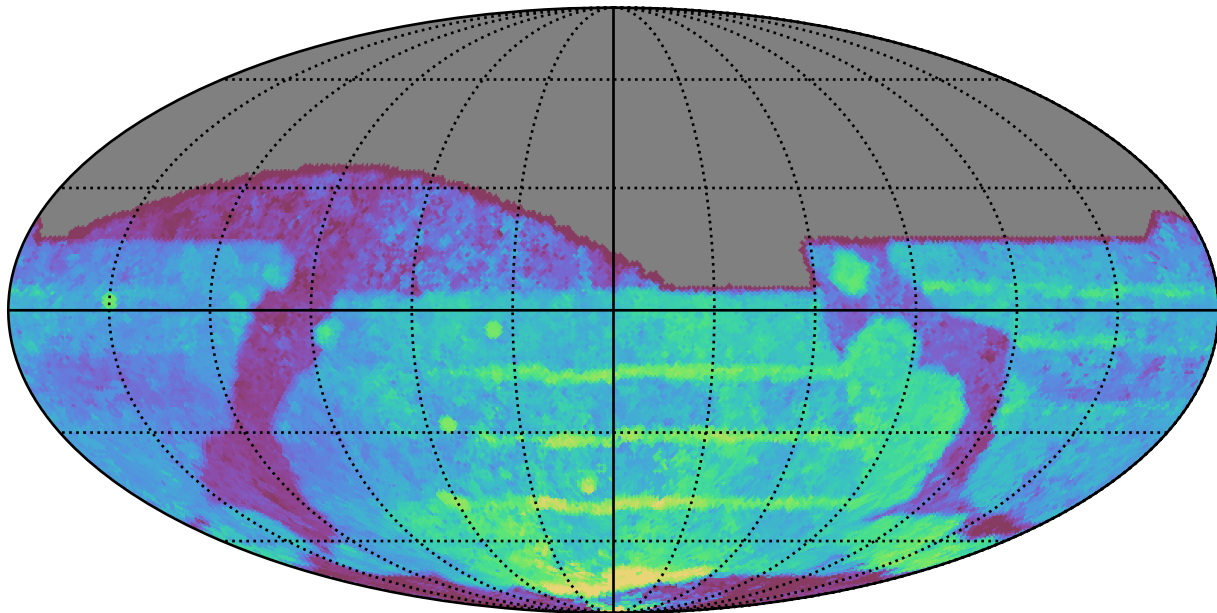
ddf_loaded_fl15_v3.4_10yrs All sky all bands: Median Season Length
