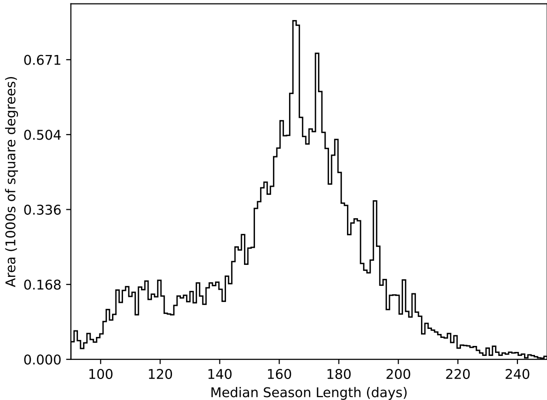
ddf_loaded_fl15_v3.4_10yrs All sky all bands: Median Season Length
