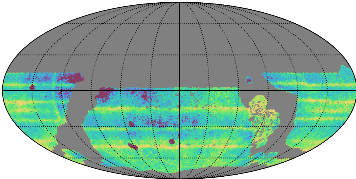
ddf_loaded_fl15_v3.4_10yrs WFD: Median Intra-Night Gap
