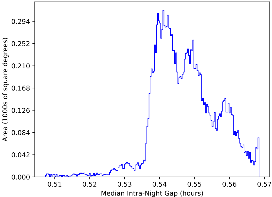
ddf_loaded_fl15_v3.4_10yrs WFD: Median Intra-Night Gap
