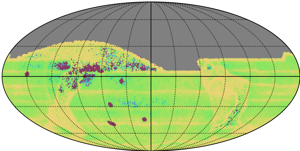
ddf_loaded_fl15_v3.4_10yrs All sky: Median Intra-Night Gap
