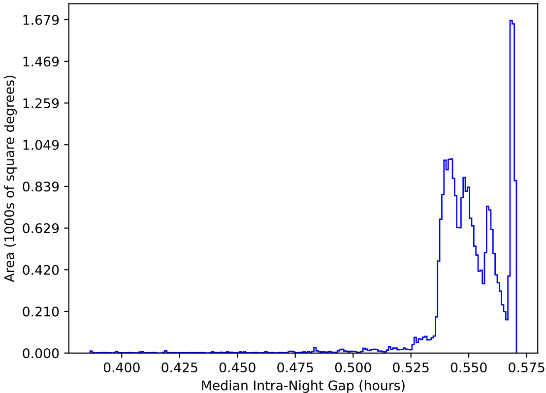
ddf_loaded_fl15_v3.4_10yrs All sky: Median Intra-Night Gap
