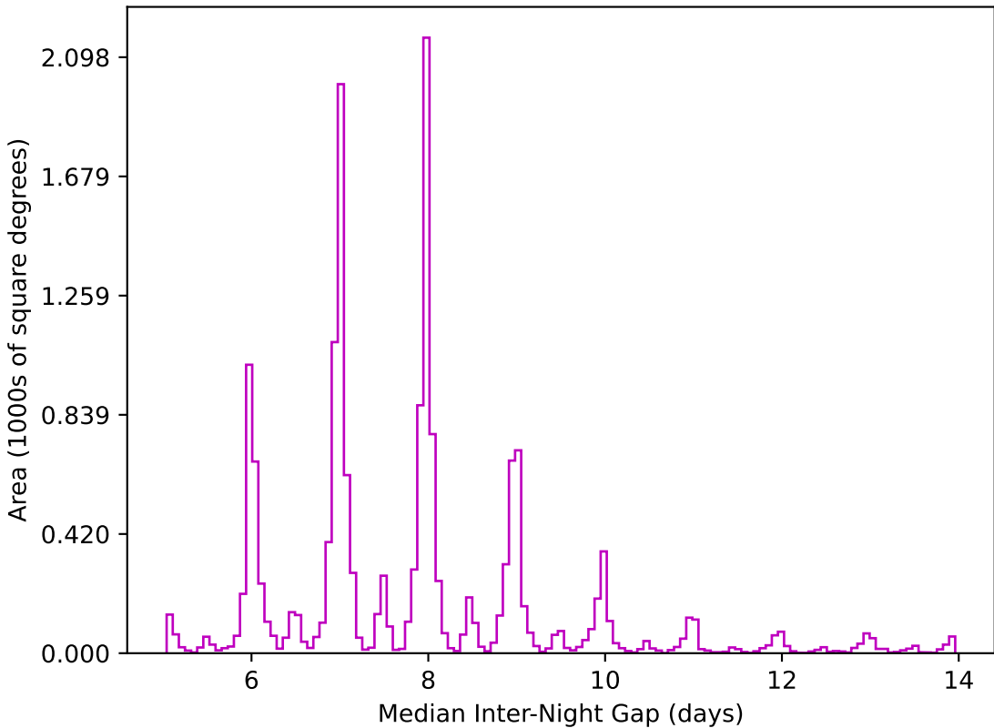
ddf_loaded_fl15_v3.4_10yrs WFD z band: Median Inter-Night Gap
