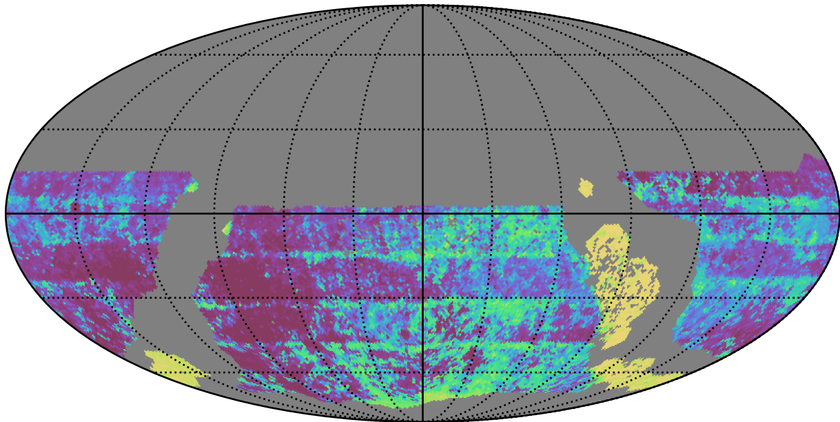
ddf_loaded_fl15_v3.4_10yrs WFD y band: Median Inter-Night Gap
