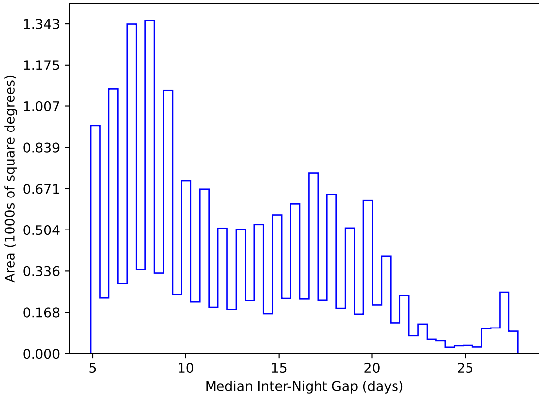
ddf_loaded_fl15_v3.4_10yrs WFD y band: Median Inter-Night Gap
