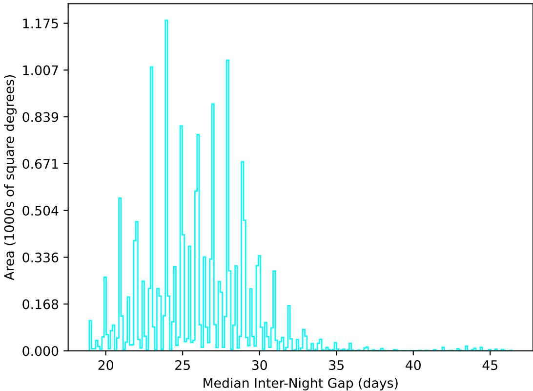
ddf_loaded_fl15_v3.4_10yrs WFD u band: Median Inter-Night Gap
