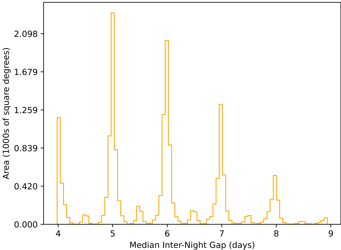
ddf_loaded_fl15_v3.4_10yrs WFD r band: Median Inter-Night Gap
