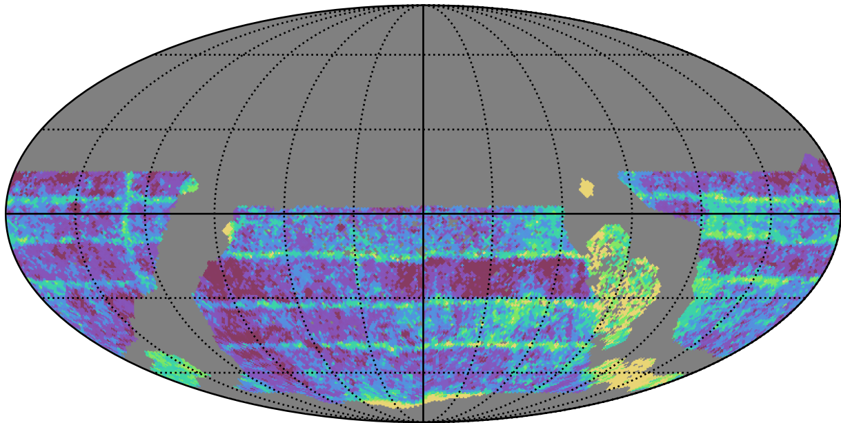
ddf_loaded_fl15_v3.4_10yrs WFD i band: Median Inter-Night Gap
