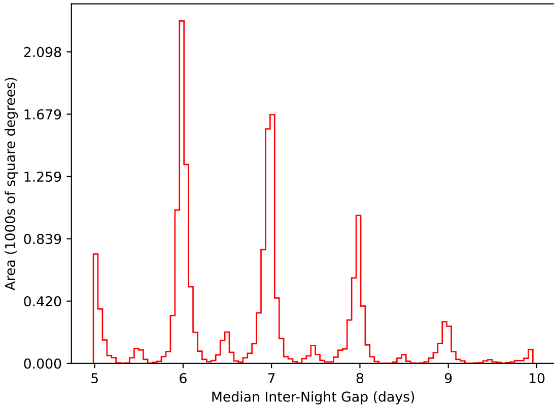
ddf_loaded_fl15_v3.4_10yrs WFD i band: Median Inter-Night Gap
