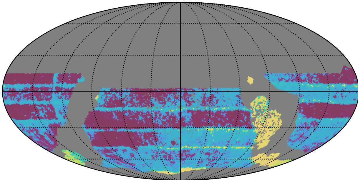
ddf_loaded_fl15_v3.4_10yrs WFD all bands: Median Inter-Night Gap
