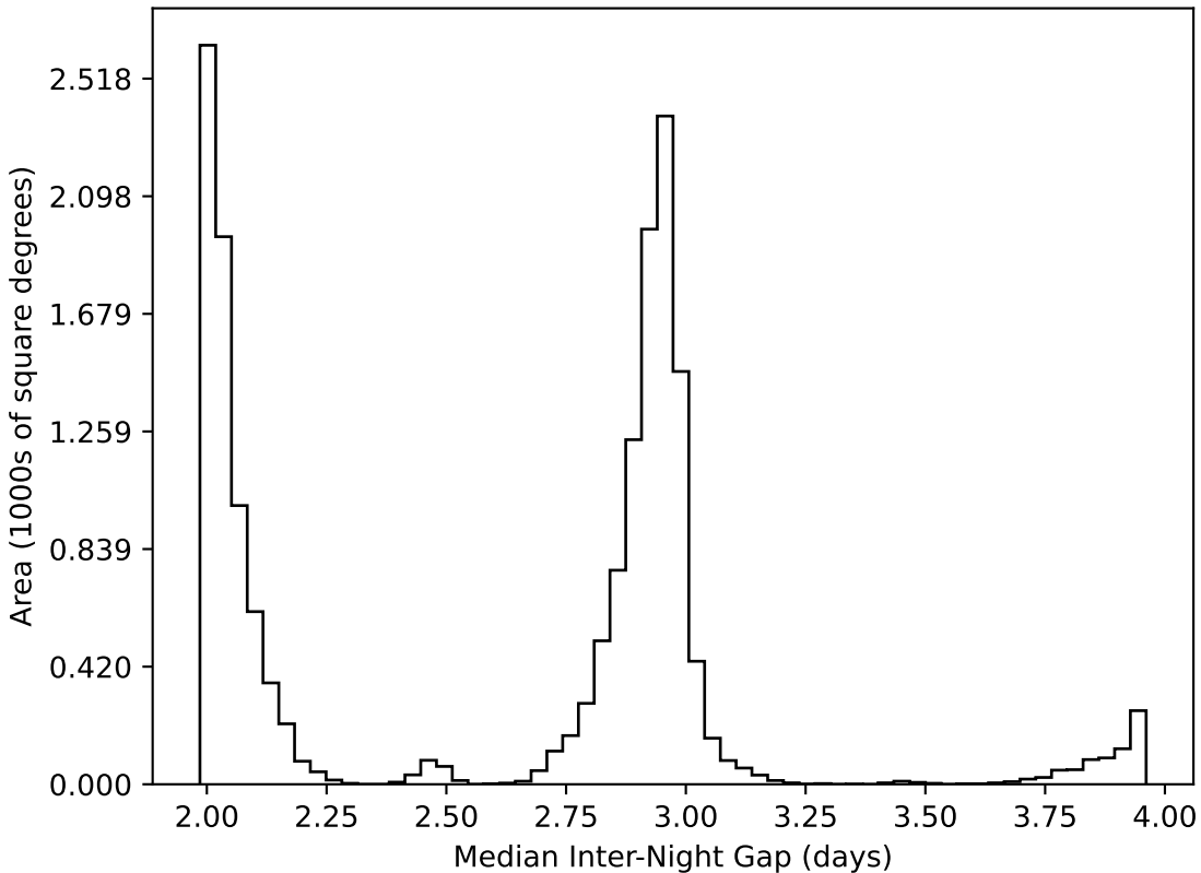
ddf_loaded_fl15_v3.4_10yrs WFD all bands: Median Inter-Night Gap
