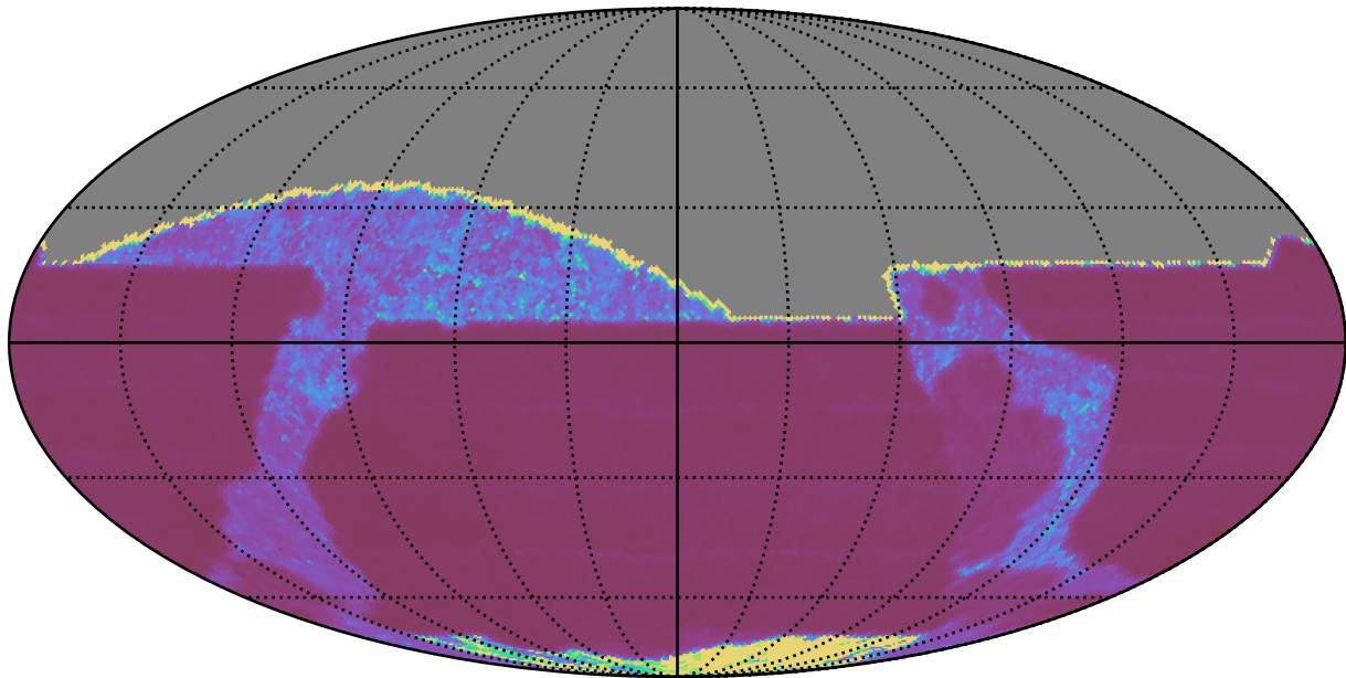
ddf_loaded_fl15_v3.4_10yrs All sky z band: Median Inter-Night Gap
